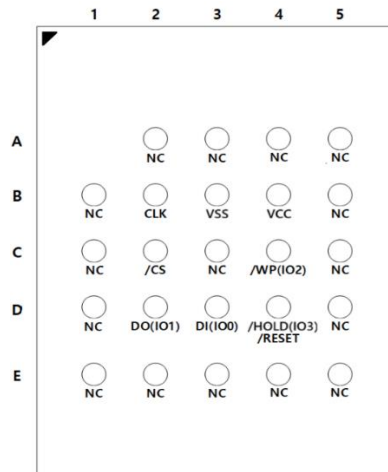
Figure 1d. 24-ball FBGA(Top View)
