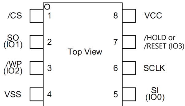
Figure 1a. 8-pin SOP 208-mil
