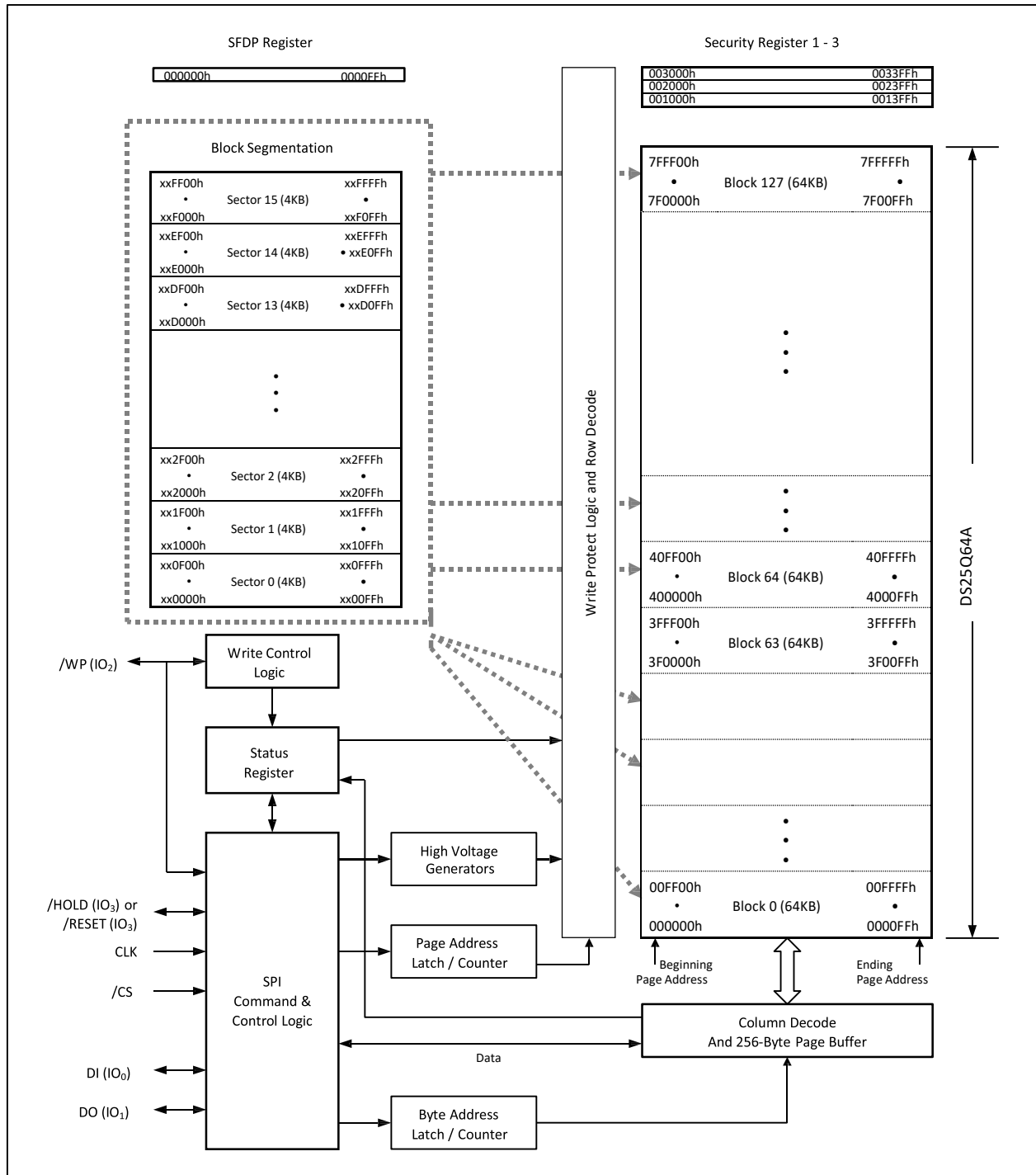
Figure 2. DS25Q64A Serial Flash Memory Block Diagram
