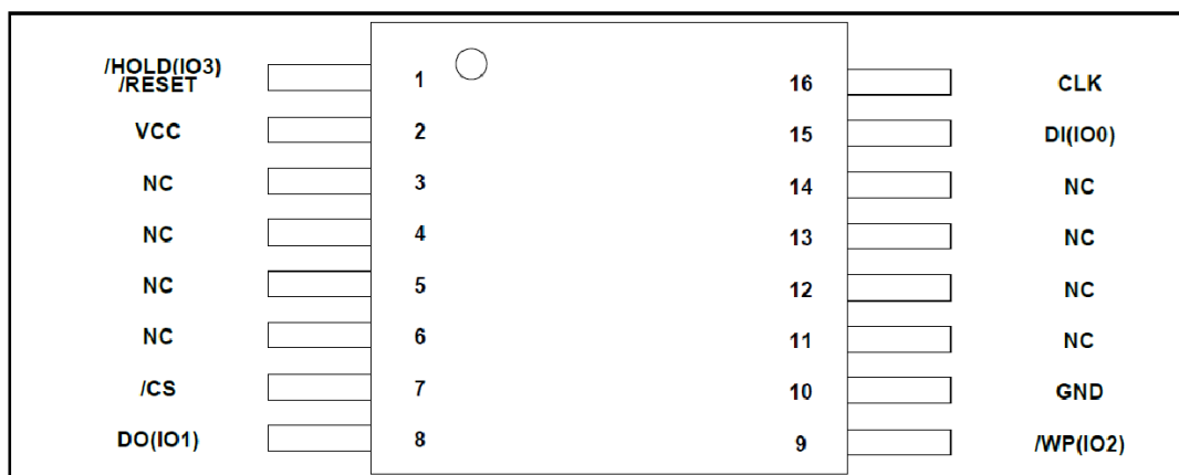
Figure 1b. 16-pin SOP 300-mil(Top View)
