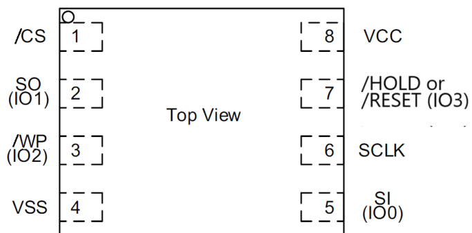
Figure 1c. 8-pad WSON 6x5-mm
